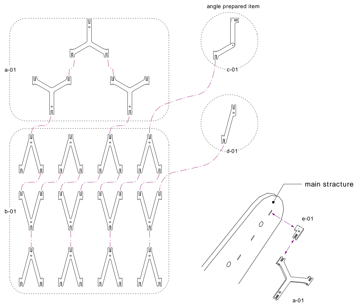
connect diagram S 1:10
