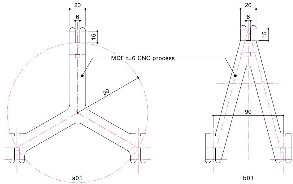
leaf form patarn S 1:3
