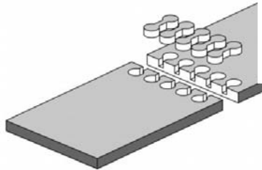
Board Lengthening with Jigsaw Keys
